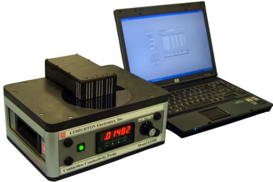
Figure 1: Model LEI88 Manual Measurement System
